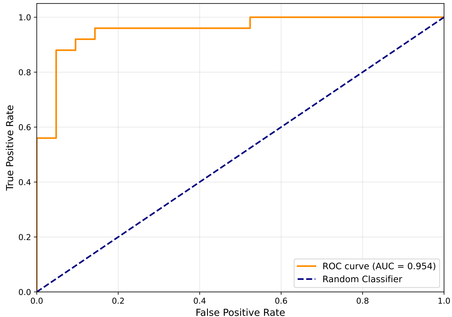
ROC Curve for Tuned Random Forest
